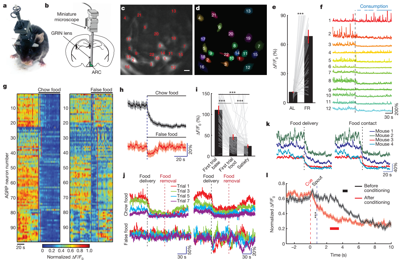
Figure 4 | Food rapidly reduces AGRP neuron activity. a, b , Configuration for deep-brain calcium imaging from AGRP neurons in freely moving mice. c, d , Image of AGRP GCaMP6f neurons ( c ) by deep-brain calcium imaging and their region of interest (ROI) spatial filters ( d ) for image analysis. Scale bar, 15 \mu m. e , Change in baseline GCaMP6 fluorescence for neurons in mice under ad libitum fed and food-restricted conditions (61 neurons, 4 mice). f , From food-restricted mice, GCaMP6f fluorescence traces from subset of individual neurons in c, d , during chow pellet food consumption. Black line, food delivery. Blue bars, food consumption. g , Normalized \text{Ca}^{2+} responses of AGRP neurons (99 neurons, 4 food-restricted mice) during exposure to a chow food pellet (left) and a false food pellet (right). Black lines, chow/false food delivery. Red lines, first contact with
