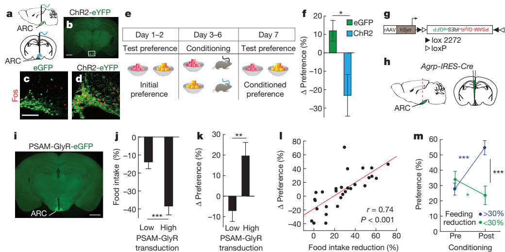
Figure 1 | AGRP neurons condition flavour preference. a , Optical fibre placement over the arcuate nucleus (ARC). b , ChR2-eYFP in AGRP neurons (box). Scale bar, 1 mm. c , d , Fos immunofluorescence following photostimulation in AGRP eGFP ( c ) or AGRP ChR2 ( d ) mice. Scale bar, 100 \mu m. e , Experimental design of conditioned flavour preference assay in ad libitum fed AGRP ChR2 or AGRP eGFP mice. f , Change in preference for flavour paired with light in AGRP eGFP and AGRP ChR2 mice (eGFP, n = 6 ; ChR2, n = 8 ). g , h , Injection of rAAV ( g ) for Cre-dependent expression of PSAM L141F -GlyR-IRES-eGFP in ( h ) AGRP neurons. i , Image of virally transduced AGRP neurons
